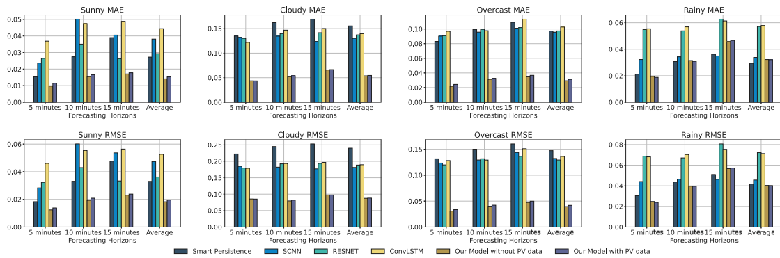
Fig. 11. Comparison of MAE and RMSE under different weather conditions.
