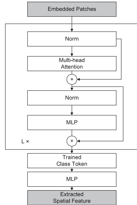
Fig. 3. The structure of the transformer encoder and MLP head [37].
