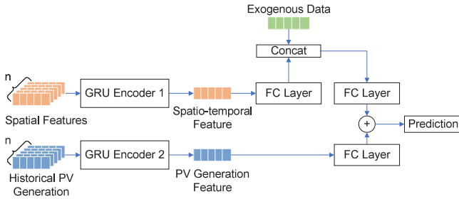
Fig. 7. Temporal processing and PV generation prediction structure.
