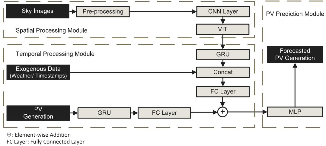
Fig. 1. Overall structure of the proposed PV forecasting framework.
