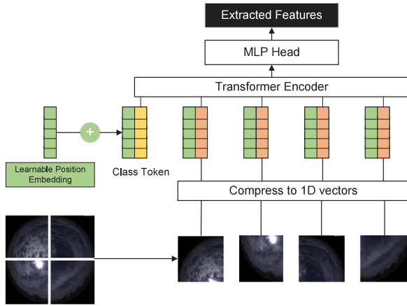
Fig. 2. ViT-based embedding structure.
