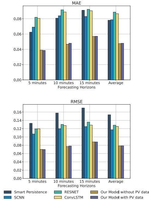
Fig. 9. Comparison of error metrics on different time horizons.
