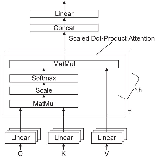
Fig. 4. The multi-head self-attention structure [37].
