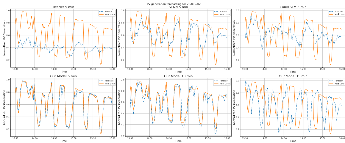
Fig. 12. Comparison of predictions and ground truth.
