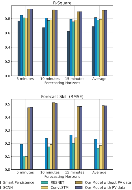
Fig. 10. Comparison of R-square and FS metrics on different time horizons.
